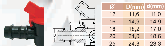
Indented Φις
